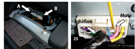
Pictures of amplifier in Land Cruiser
